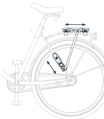
Step 10: Position the footrests and mounting frame
