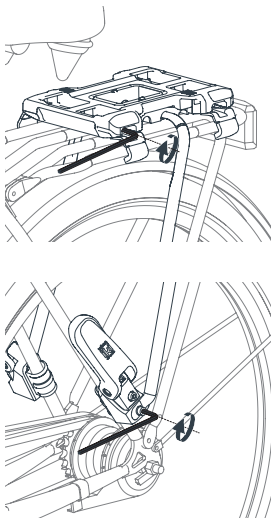
Step 11: Tighten the footrests and mounting frame
