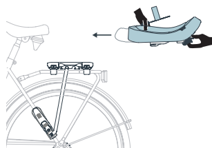
2. Slide the Junior seat in a horizontal position over the mounting frame
