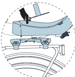
2. Slide the Junior seat in a horizontal position over the mounting frame
