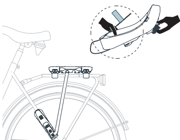
Step 12: Place the seat on the carrier
